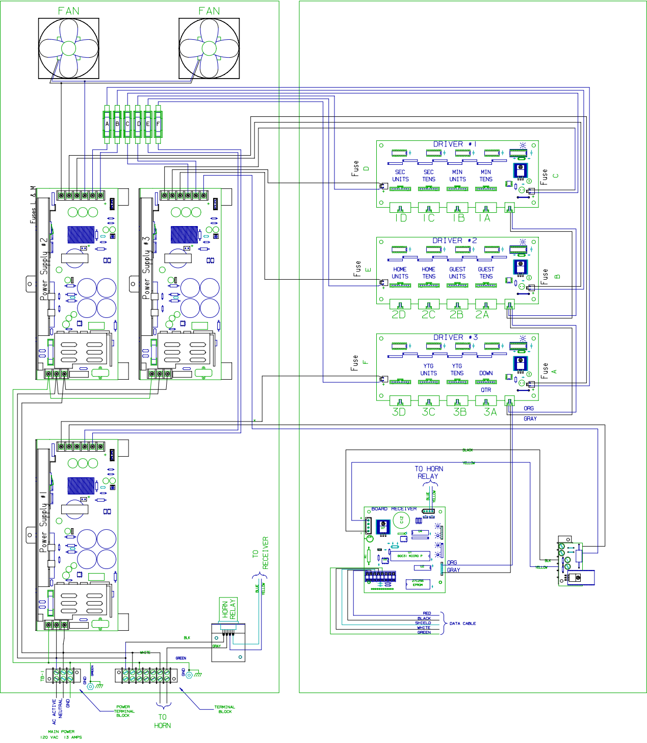
CONTROLLER ASSEMBLY
