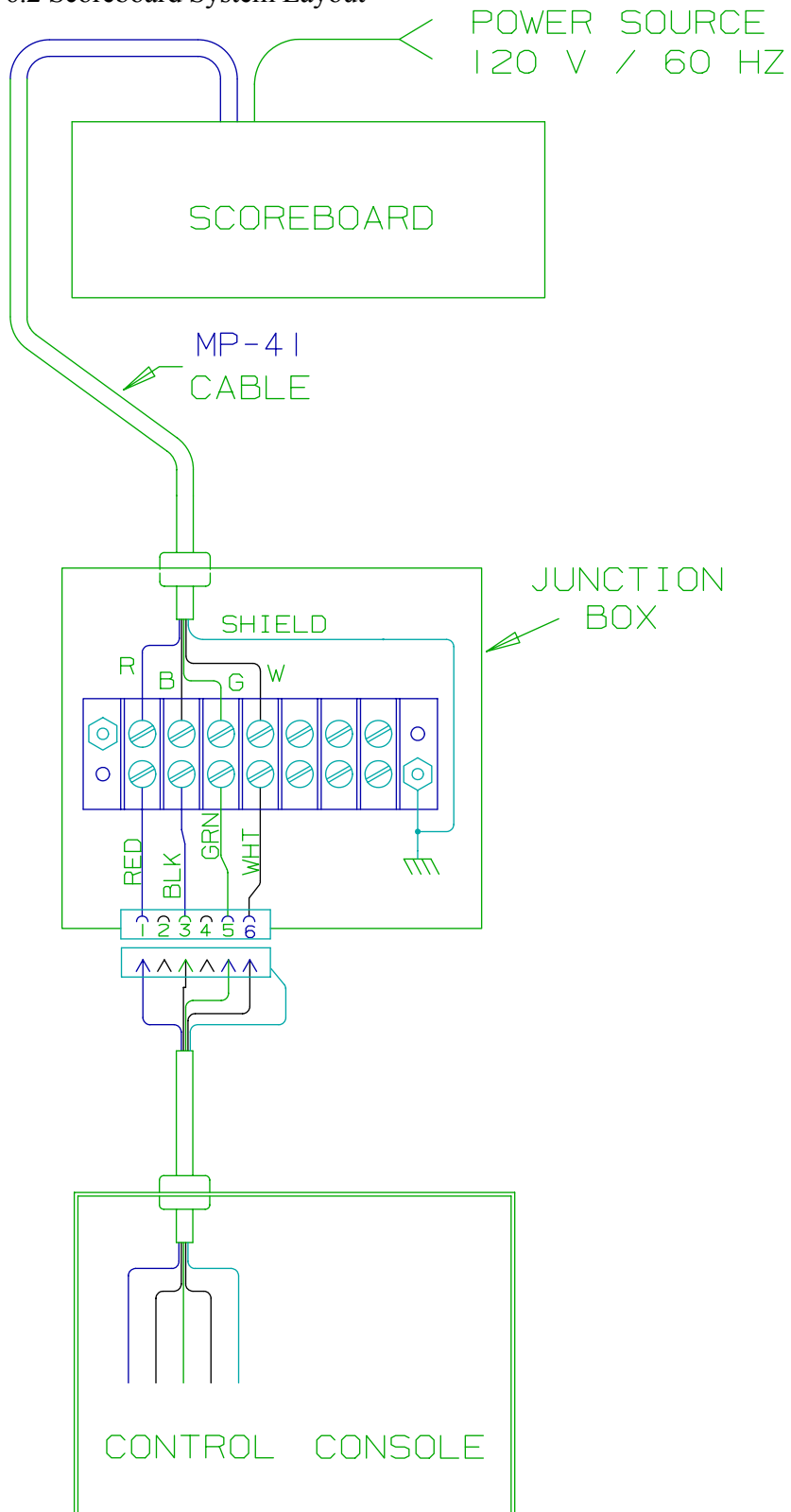
figure 4 SYSTEM LAYOUT
