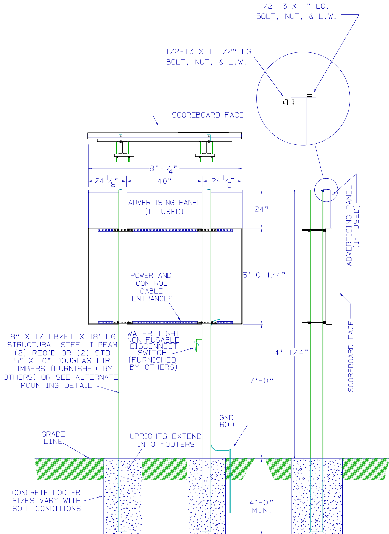
6.7 Installation Drawing Cont.
