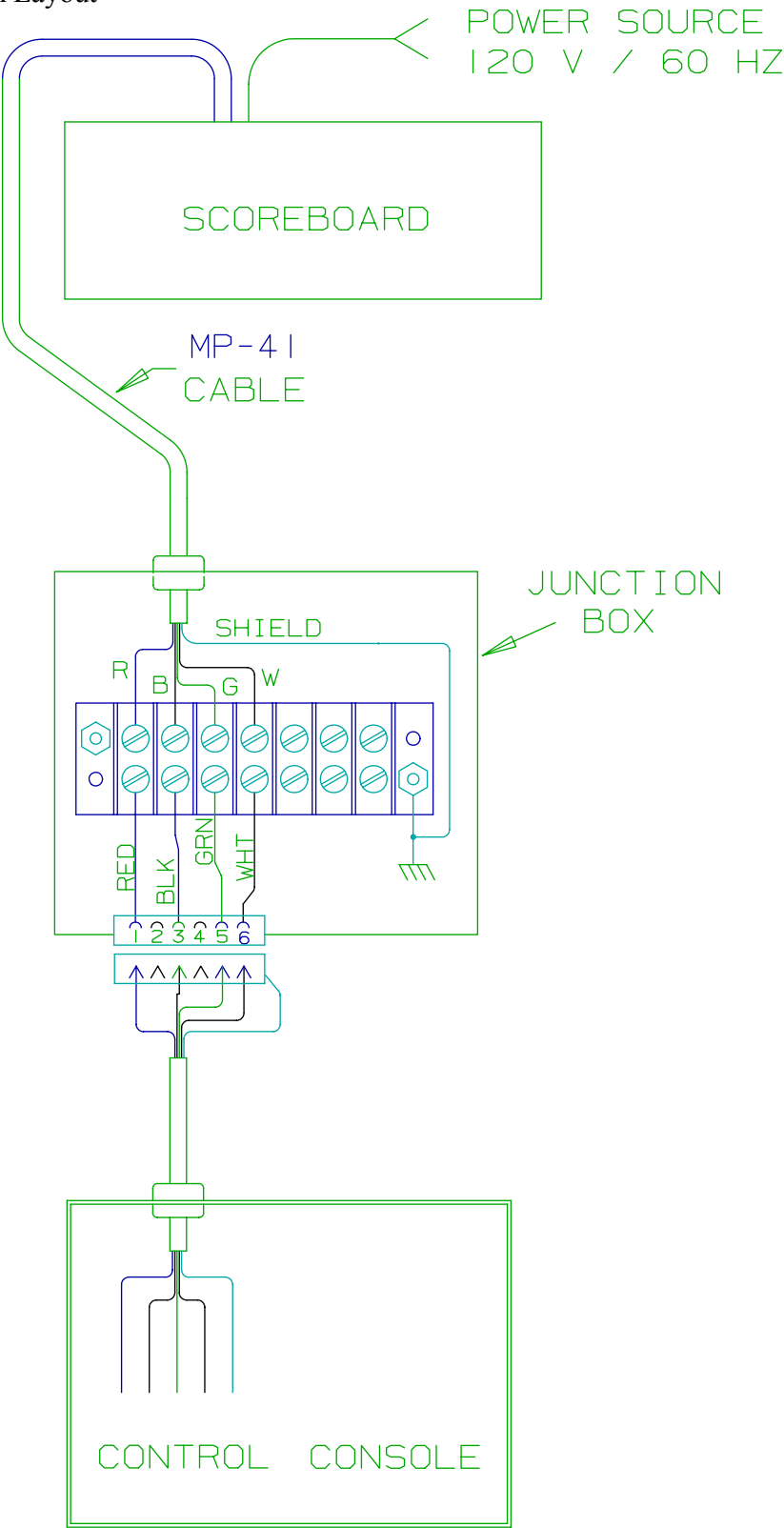
figure 4 SYSTEM LAYOUT
