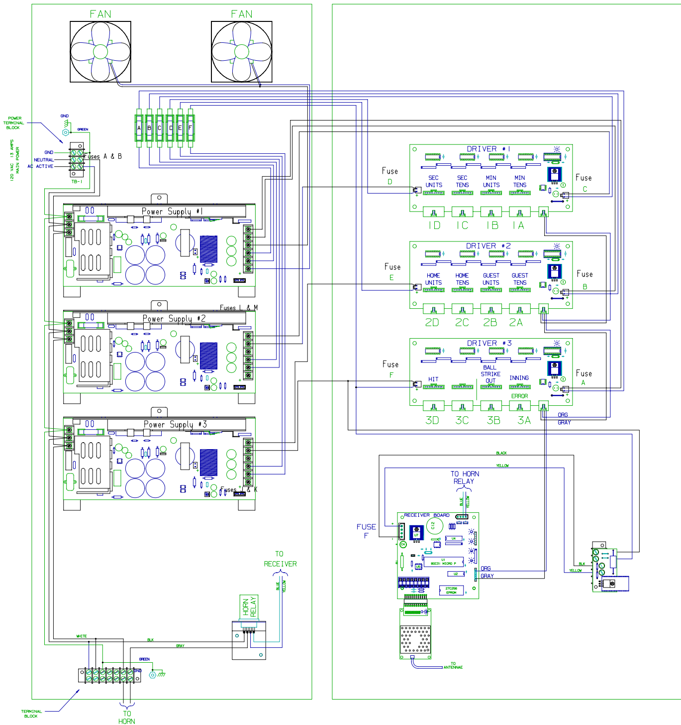
CONTROLLER ASSEMBLY
