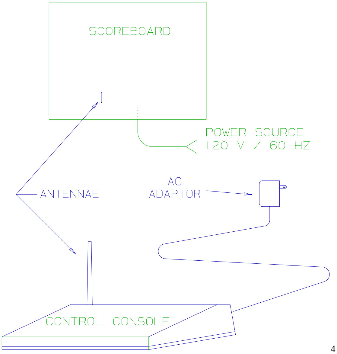
figure 4 SYSTEM LAYOUT
