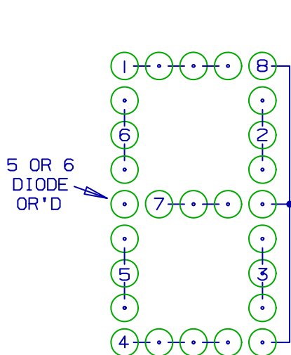
MICROPROCESSOR 5 X 9 (8 BIT) LED PATTERN
