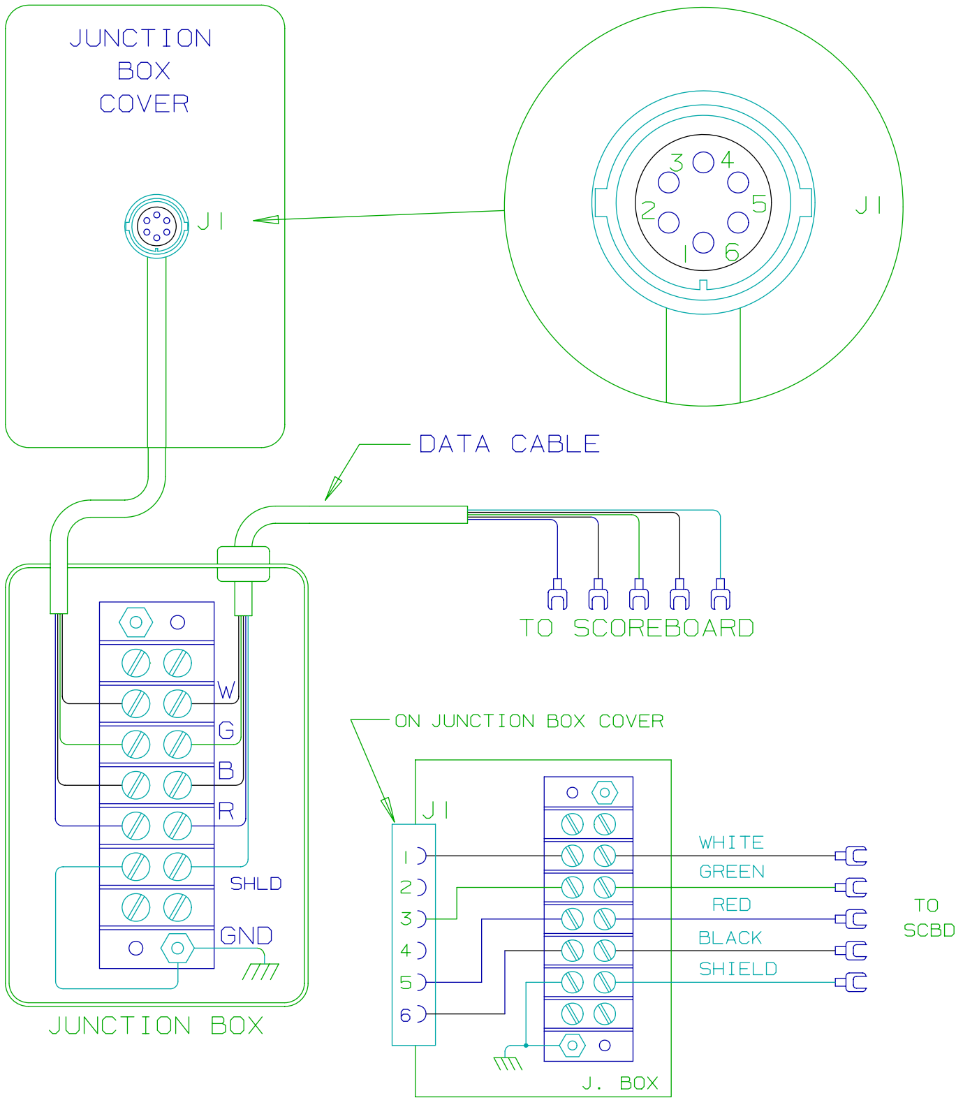
JUNCTION BOX WIRING
