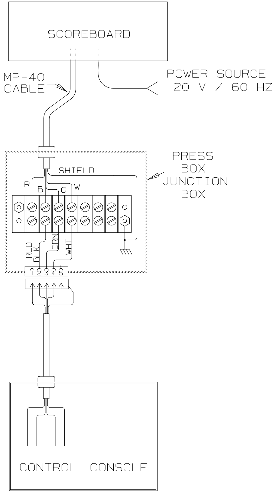
SYSTEM LAYOUT
