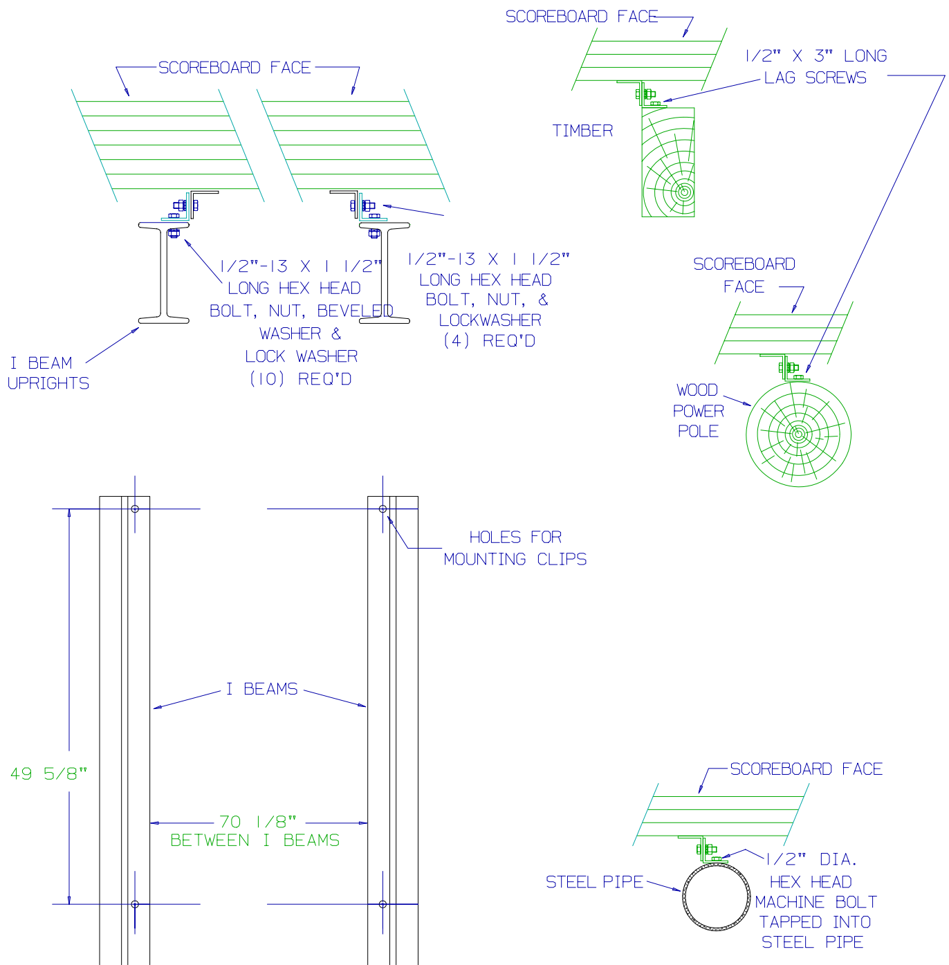
FRONT VIEW MOUNTING DETAIL
