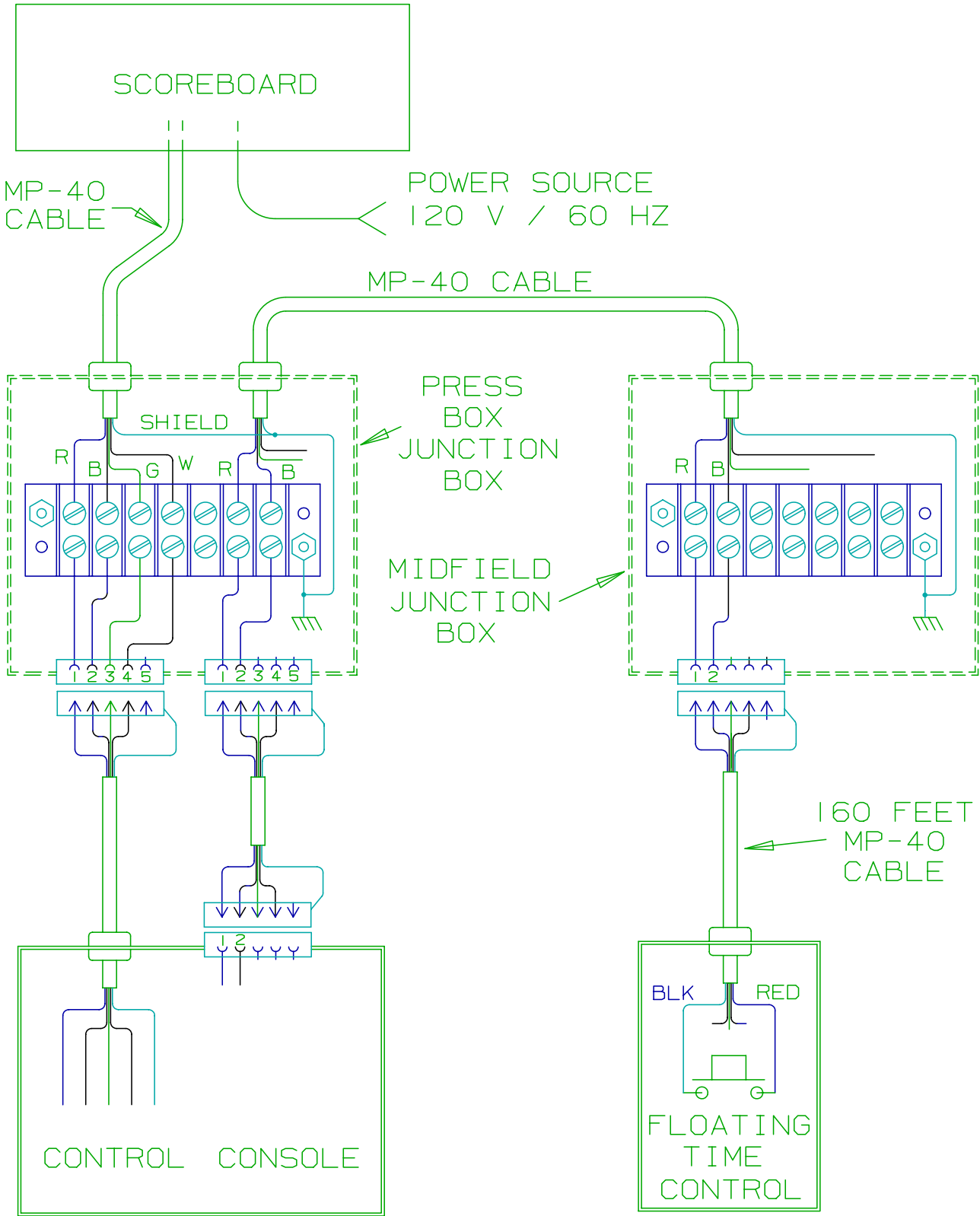
figure 4 SYSTEM LAYOUT
