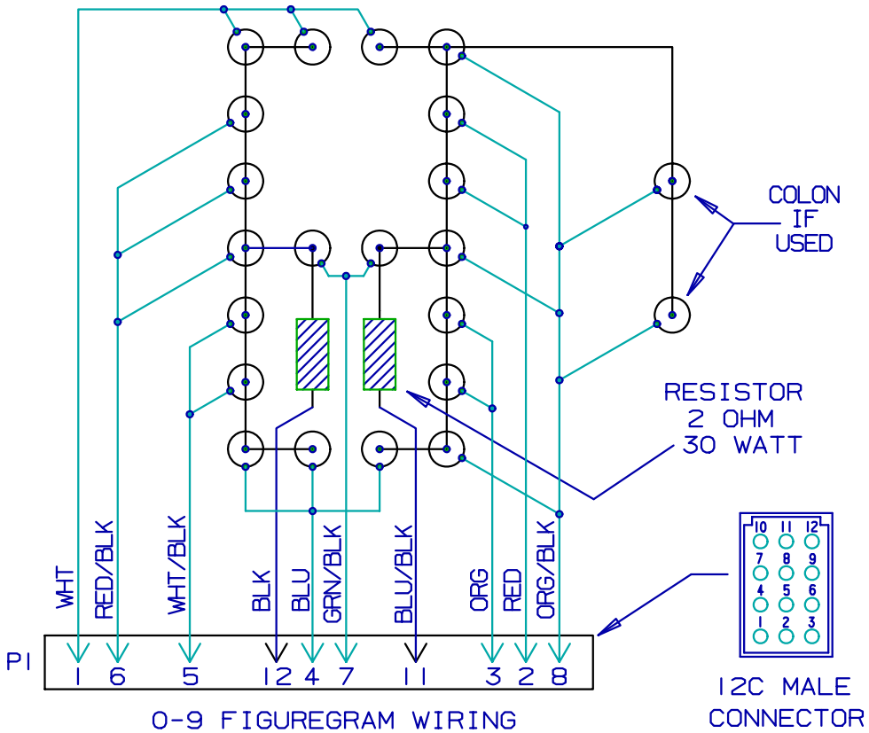
FIGUREGRAM WIRING
