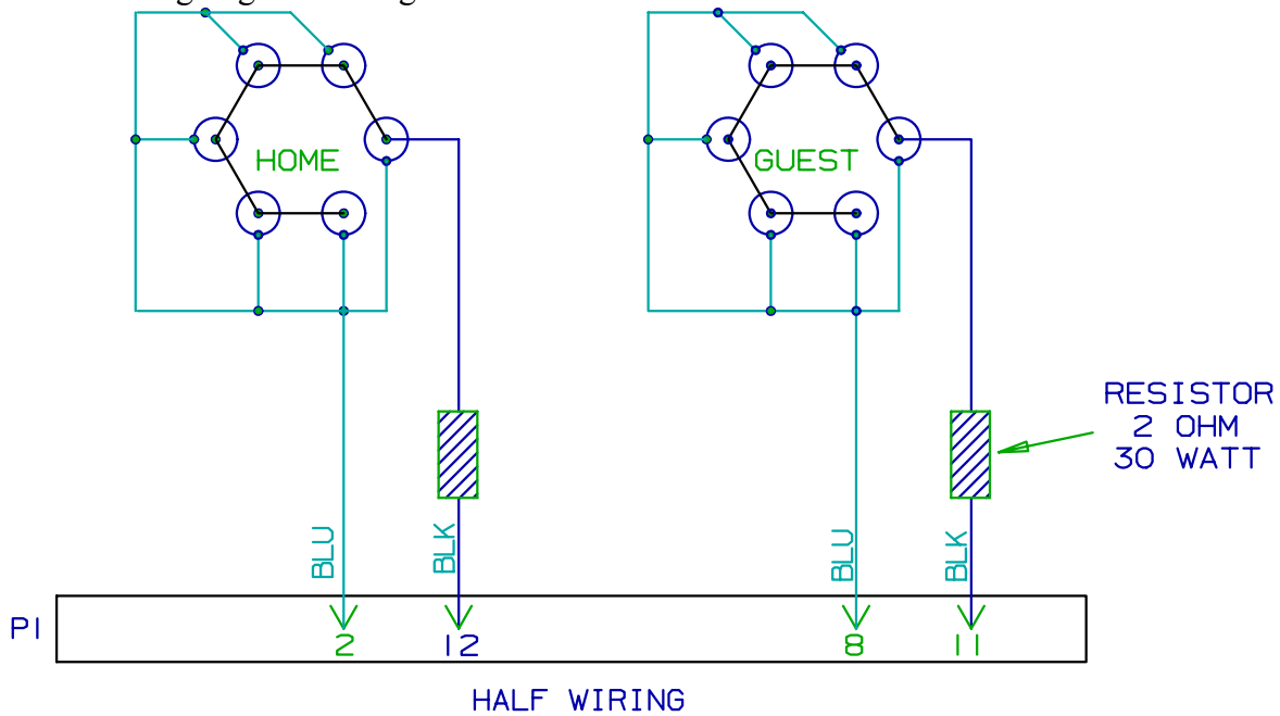
6.7 Figuregram Wiring
