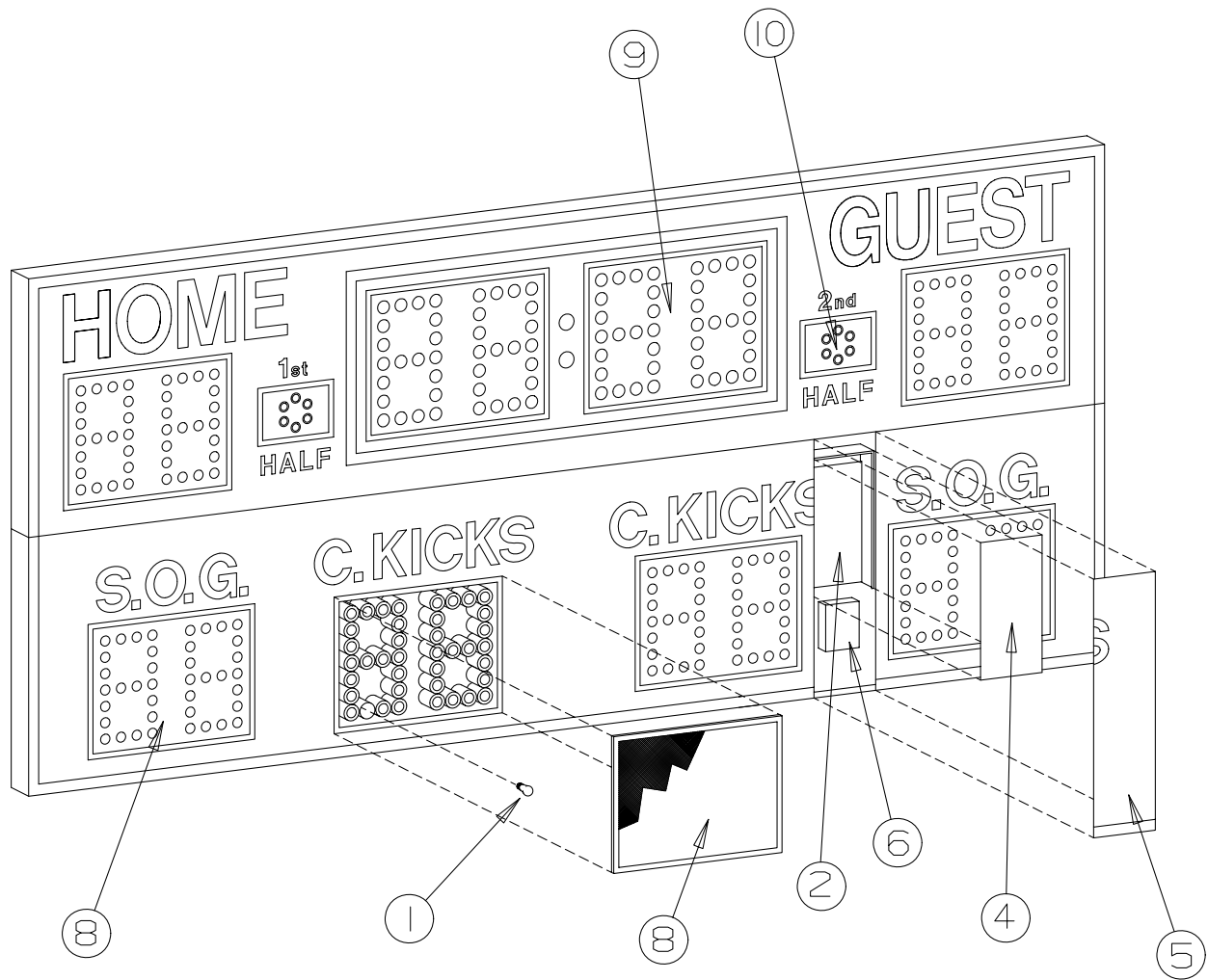
figure 1 DISPLAY ASSEMBLY
