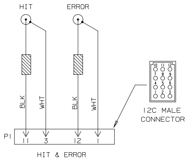
FIGUREGRAM WIRING
