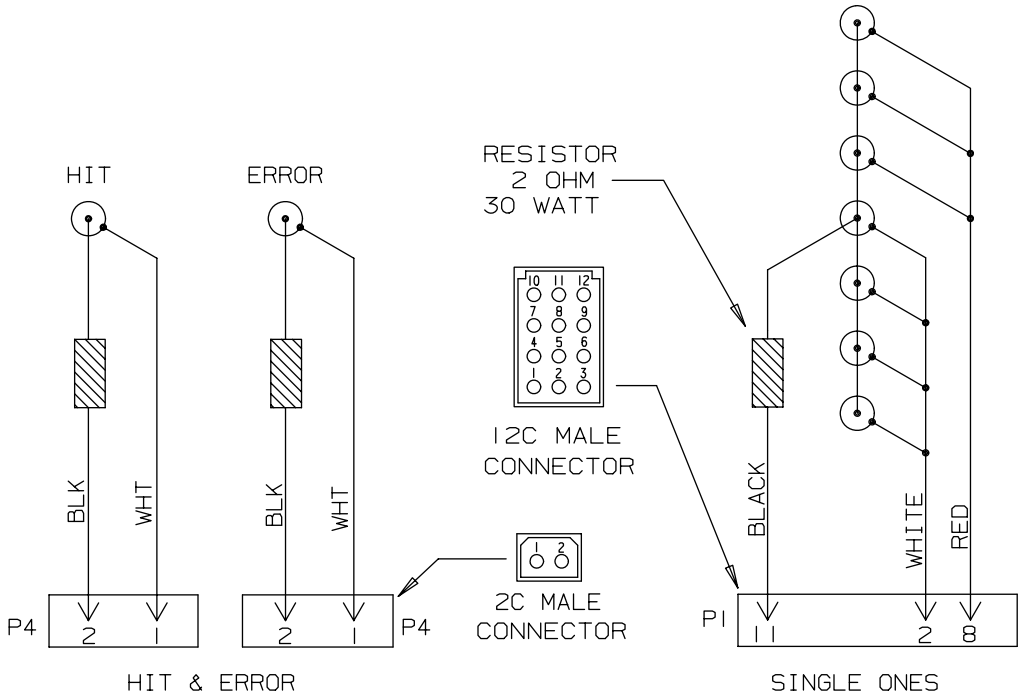
FIGUREGRAM WIRING
