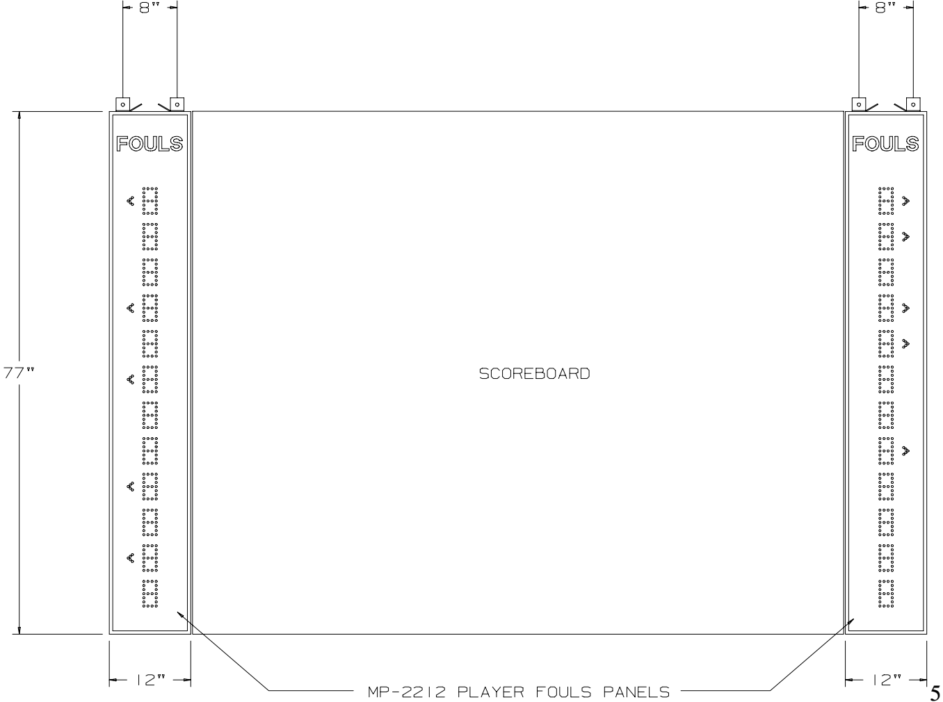
INSTALLATION DRAWING
