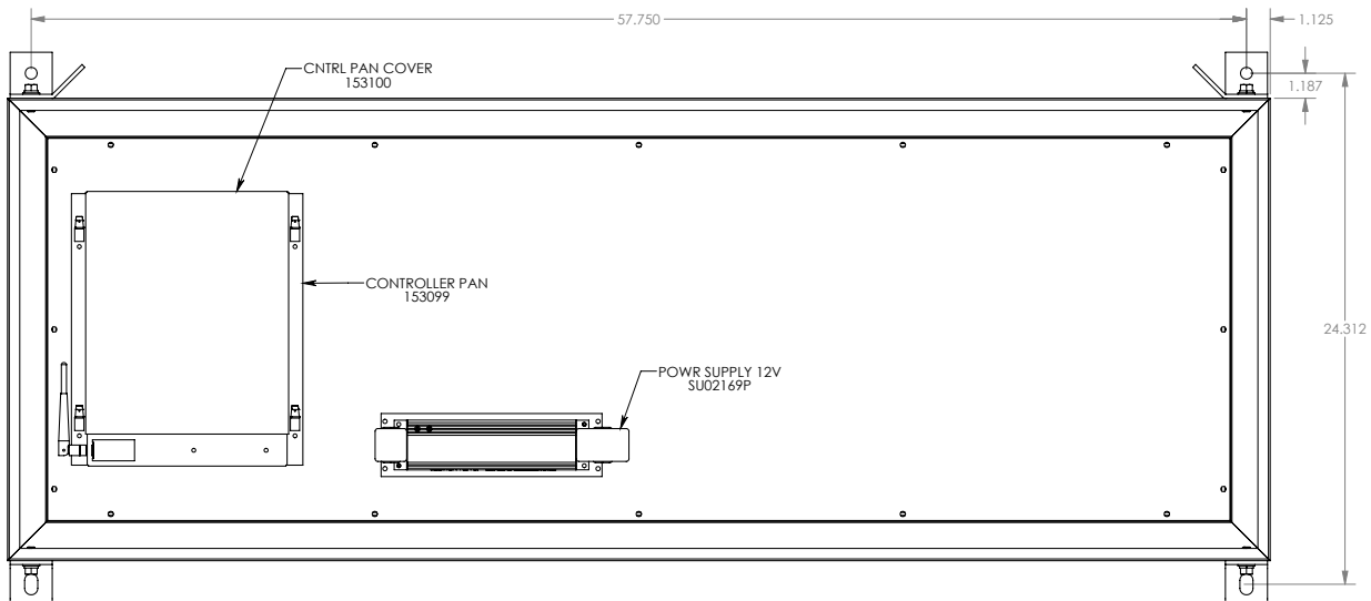
FRONT VIEW (DOOR & FACE REMOVED)
