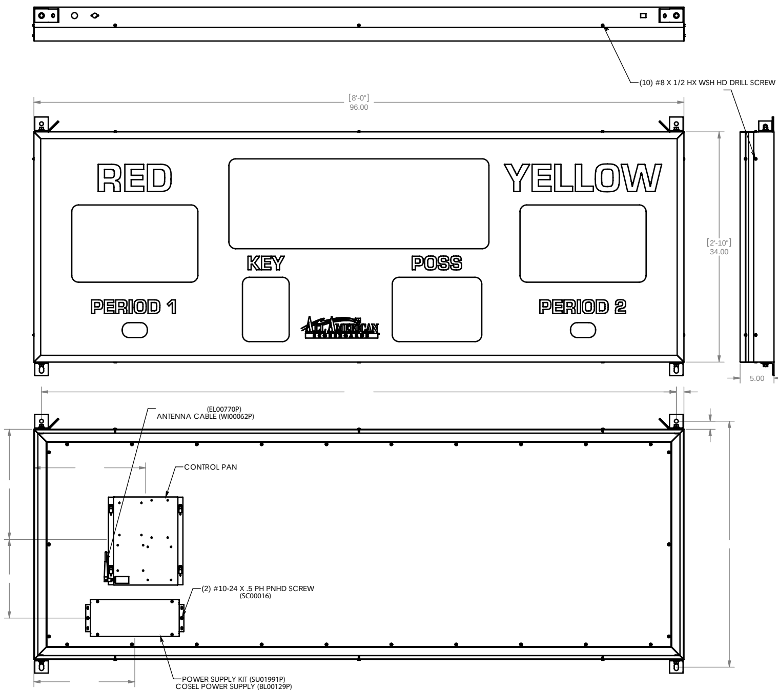
FRONT VIEW (DOOR & FACE REMOVED)
