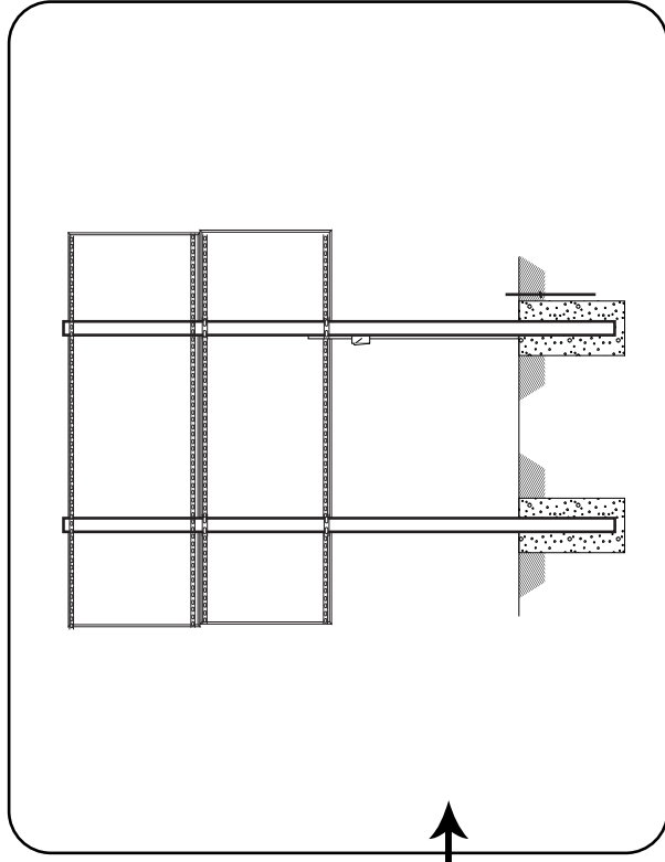
Typical 2 Cabinet Scoreboard Installation Illustration
